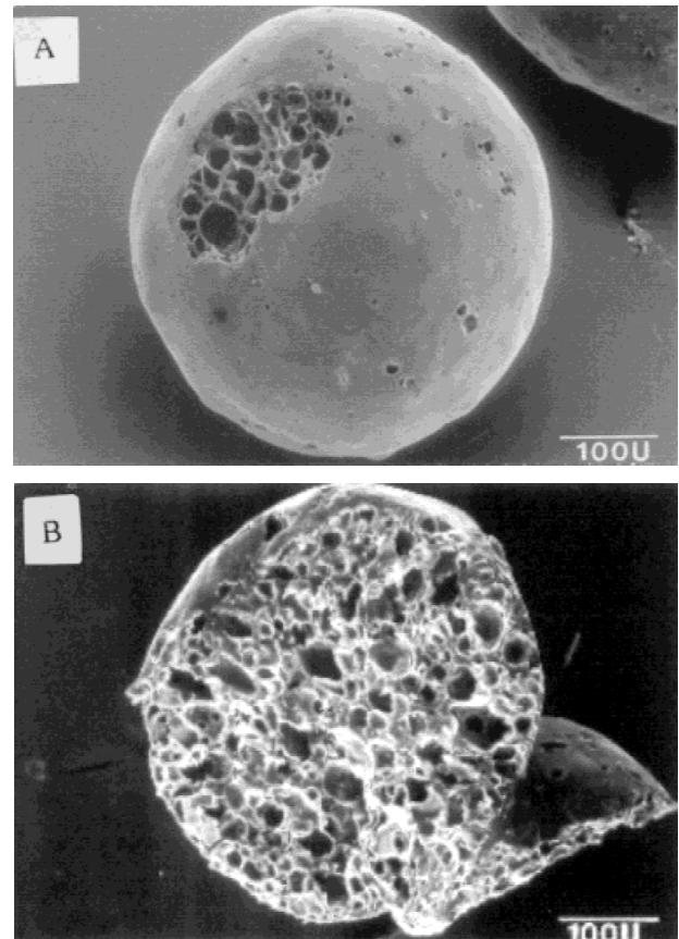
Fig. 5. (a) Microspheres from the same preparation as Figure 4 after 28 days in vitro ganciclovir release study in PBS ( \times 160 ). (b). View of a fragmented microsphere treated as (a) ( \times 160 ).
